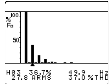
Harmonics Display
